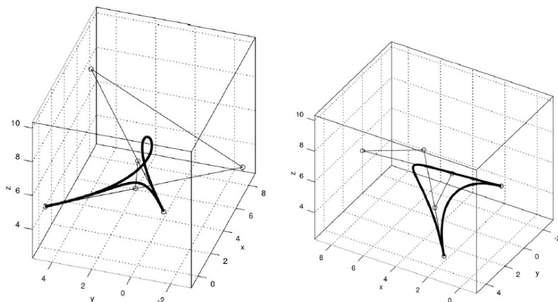
Figure 4. Example of interpolation in case there are two solutions: points \mathbf{p}_0 = (1, 1, 3)^T , \mathbf{p}_3 = (1, 5, 4)^T and tangents \mathbf{e}_{\mathbf{t}_0} = \left(\frac{3}{\sqrt{22}}, \frac{3}{\sqrt{22}}, \frac{2}{\sqrt{22}}\right)^T , \mathbf{e}_{\mathbf{t}_2} = \left(-\frac{3}{5}, \frac{4}{5}, 0\right)^T , from two perspectives.
