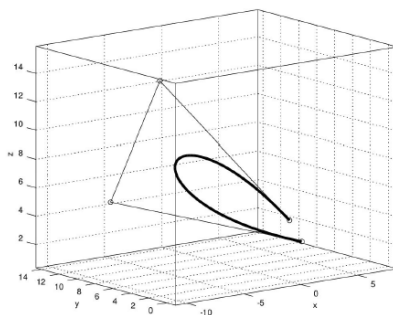
Figure 3. Example of interpolation, when there is just one solution: points \mathbf{p}_0 = (-1, -1, 5)^T , \mathbf{p}_3 = (4, 4, 2)^T and
