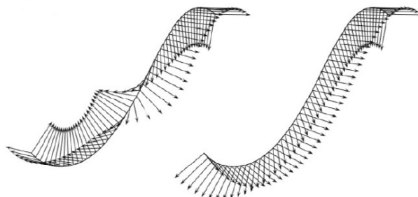
Figure 2. Frenet frame (left) and rotation-minimizing frame (right).
